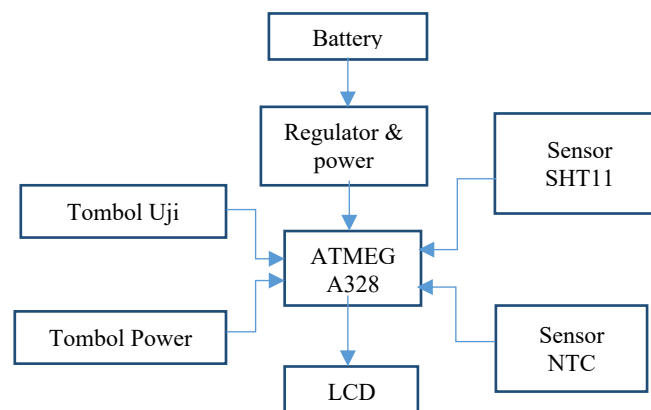
Gambar 2. Diagram blok alat ukur kadar air biji kopi
